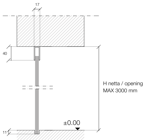
Profilo Orizzontale / A soffitto Horizontal Fixed Profile / Ceiling-mounted
