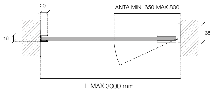
Profilo Verticale / A parete Vertical Profile / Wall-mounted
