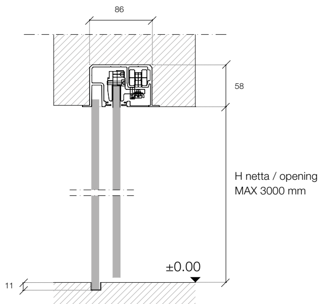
Binario Scorrevole / A incasso Sliding Rail / Recessed
