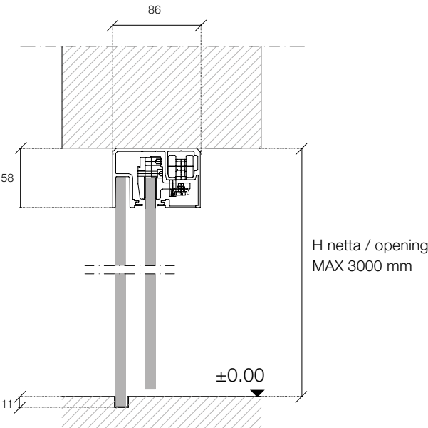
Binario Scorrevole / A soffitto Sliding Rail / Recessed
