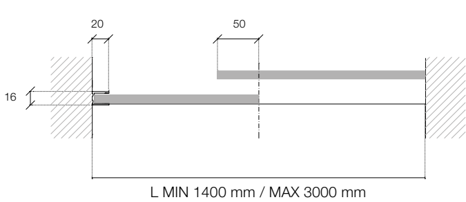
Profilo Verticale / A parete Exterior Vertical Profile / Wall-mounted
