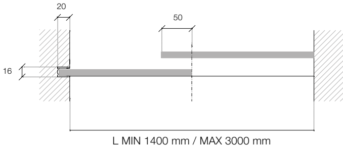
Profilo Verticale / A incasso Exterior Vertical Profile / Recessed
