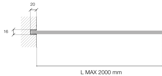
Profilo Verticale / A incasso Vertical Profile / Recessed
