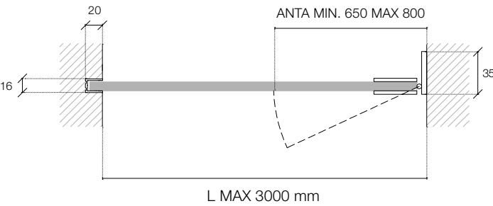
Profilo Verticale / A incasso Vertical Profile / Recessed
