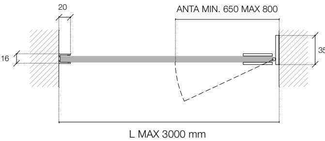
Profilo Verticale / A parete Vertical Profile / Wall-mounted
