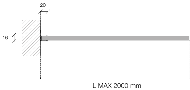
Profilo Verticale / A parete Vertical Profile / Wall-mounted
