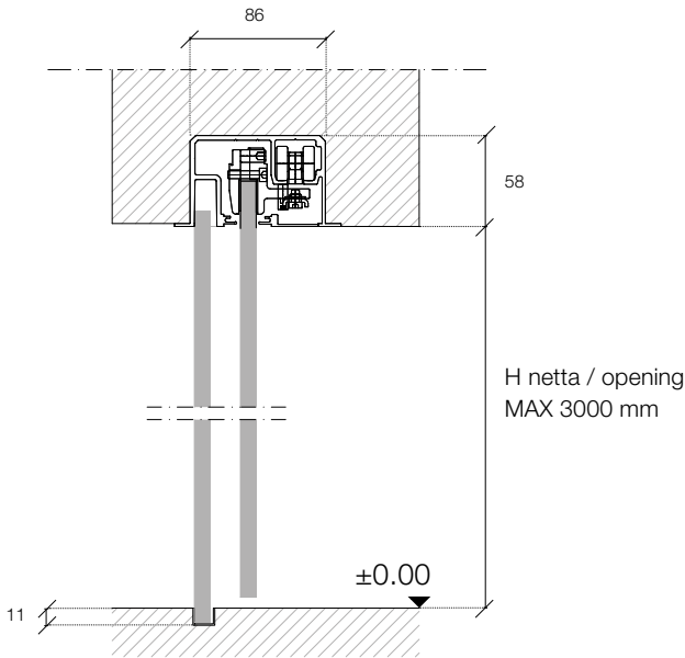
Binario Scorrevole / A incasso Sliding Rail / Recessed
