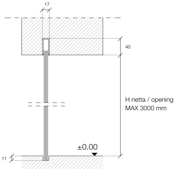
Profilo Orizzontale / A incasso Horizontal Fixed Profile / Recessed
