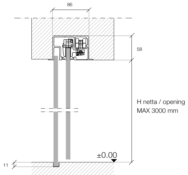
Binario Scorrevole / A incasso Sliding Rail / Recessed
