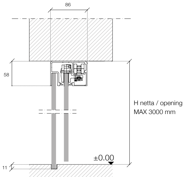
Binario Scorrevole / A soffitto Sliding Rail / Recessed
