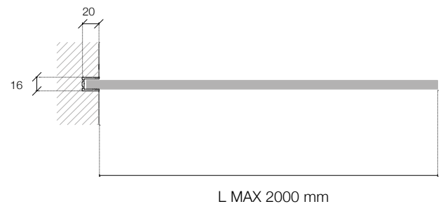
Profilo Verticale / A incasso Vertical Profile / Recessed
